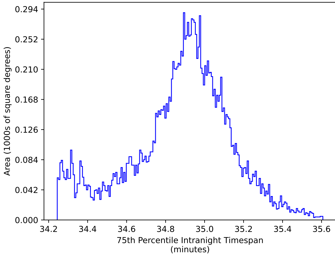
ddf_acor_sf15_Isf40_Isr20_v3.4_10yrs WFD all bands: 75th Percentile Intranight Timespan
