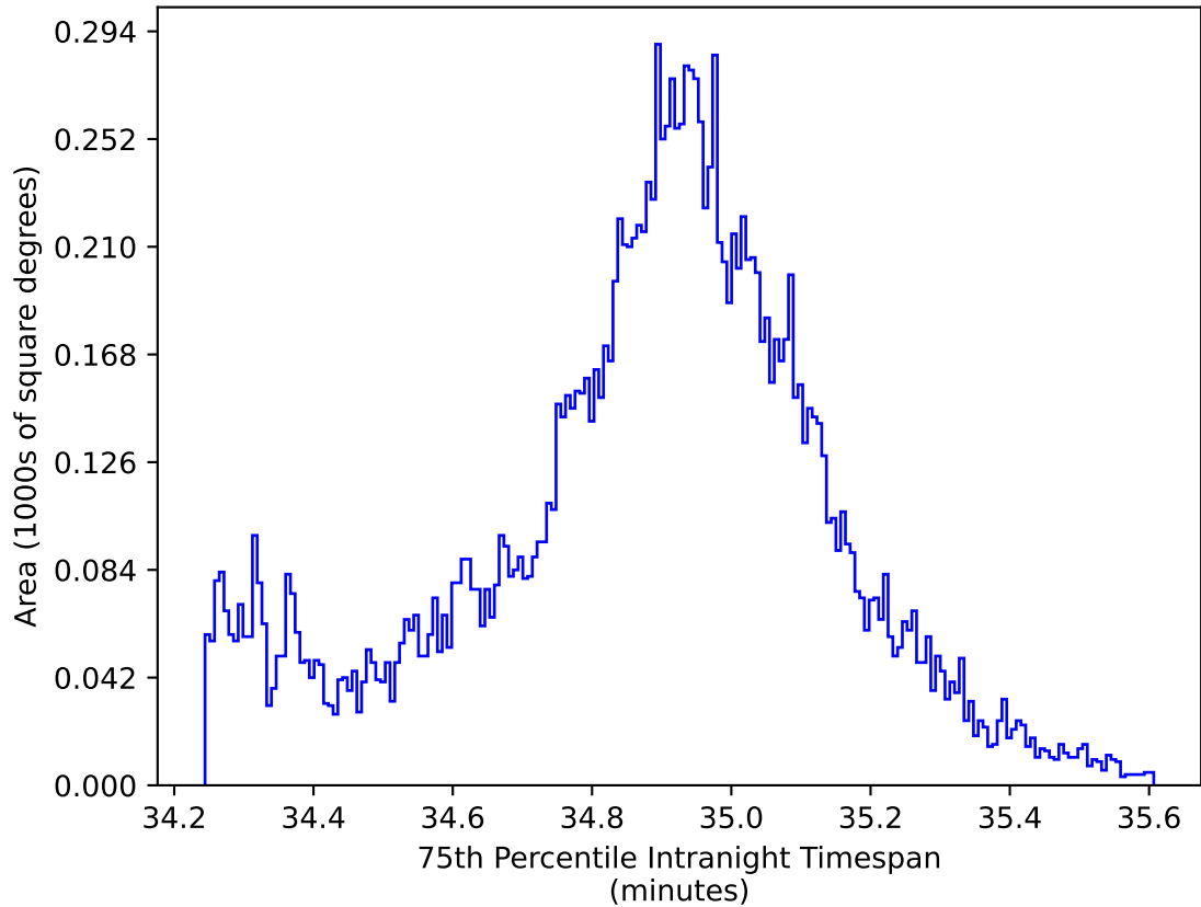
ddf_acor_sf15_lsf40_lsr20_v3.4_10yrs WFD: 75th Percentile Intranight Timespan
