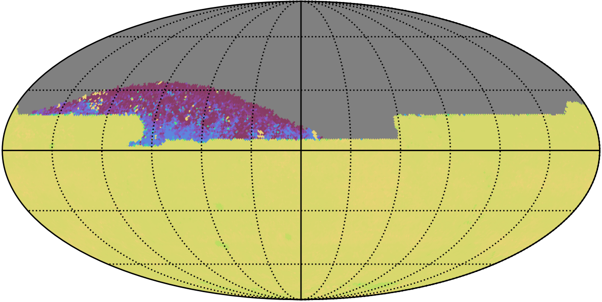
ddf_acor_sf15_lsf40_lsr20_v3.4_10yrs All sky zy bands: 75th Percentile Intranight Timespan
