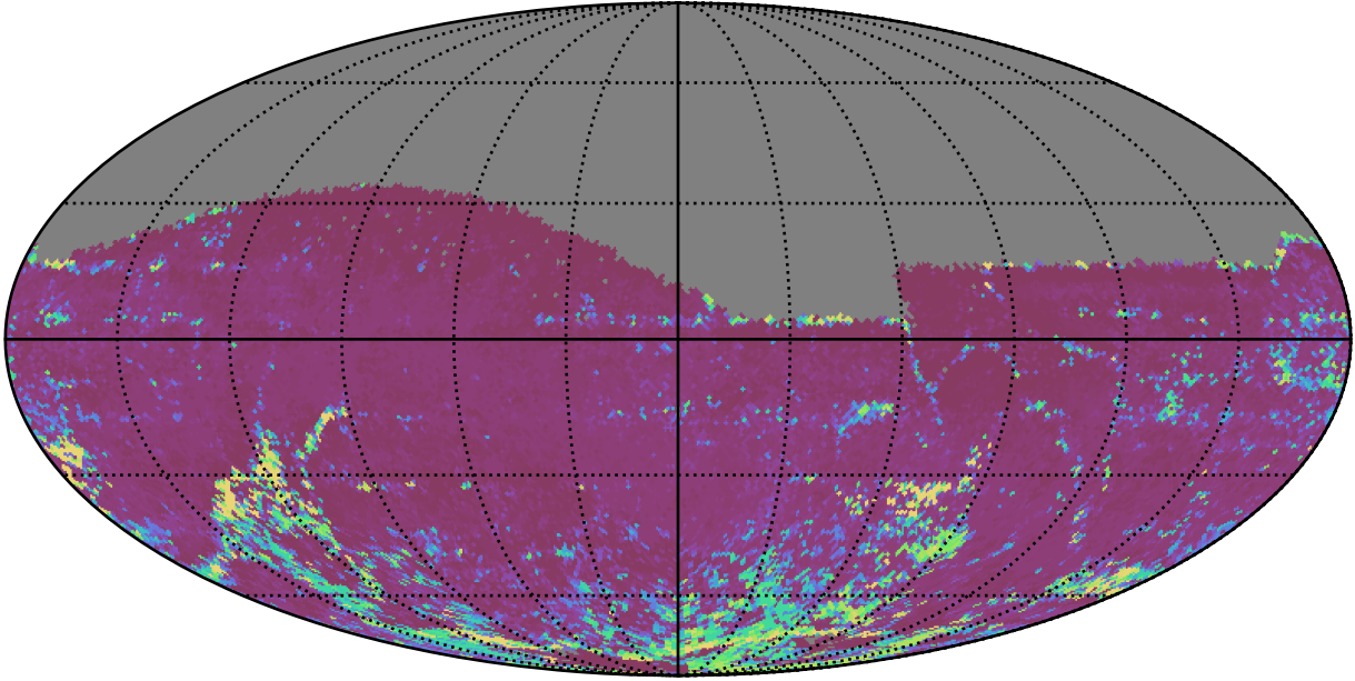
ddf_acor_sf15_lsf40_lsr20_v3.4_10yrs All sky z band: 75th Percentile Intranight Timespan
