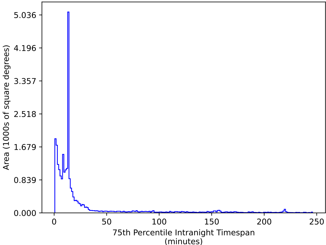
ddf_acor_sf15_lsf40_lsr20_v3.4_10yrs All sky z band: 75th Percentile Intranight Timespan
