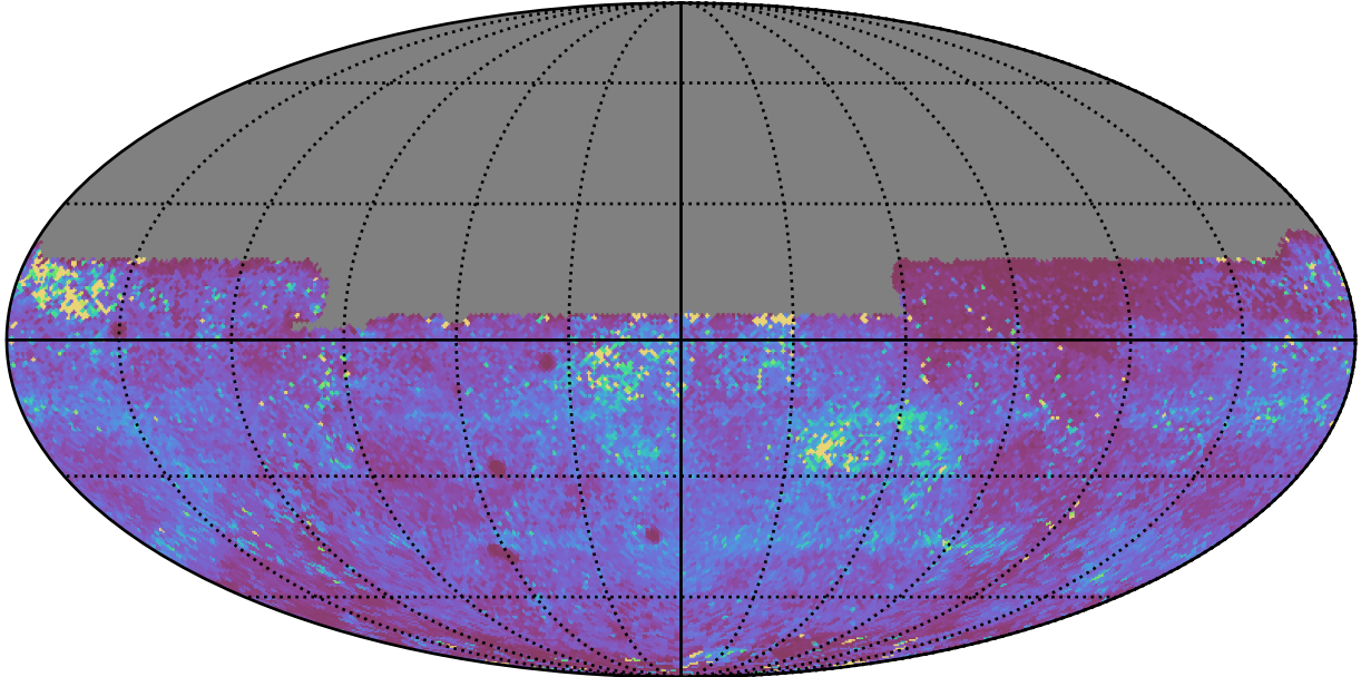
ddf_acor_sf15_lsf40_lsr20_v3.4_10yrs All sky y band: 75th Percentile Intranight Timespan
