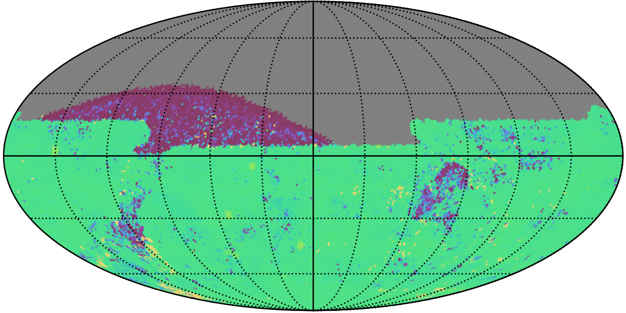
ddf_acor_sf15_lsf40_lsr20_v3.4_10yrs All sky ug bands: 75th Percentile Intranight Timespan
