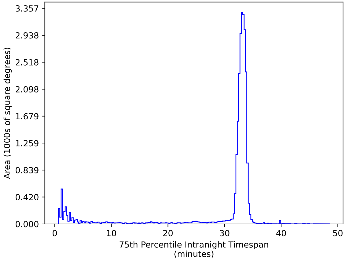
ddf_acor_sf15_lsf40_lsr20_v3.4_10yrs All sky ug bands: 75th Percentile Intranight Timespan
