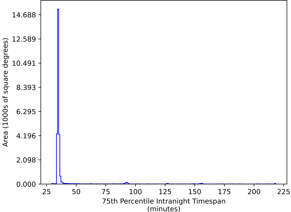
ddf_acor_sf15_lsf40_lsr20_v3.4_10yrs All sky ri bands: 75th Percentile Intranight Timespan
