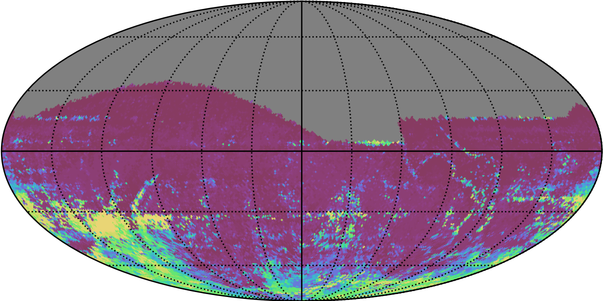
ddf_acor_sf15_lsf40_lsr20_v3.4_10yrs All sky r band: 75th Percentile Intranight Timespan
