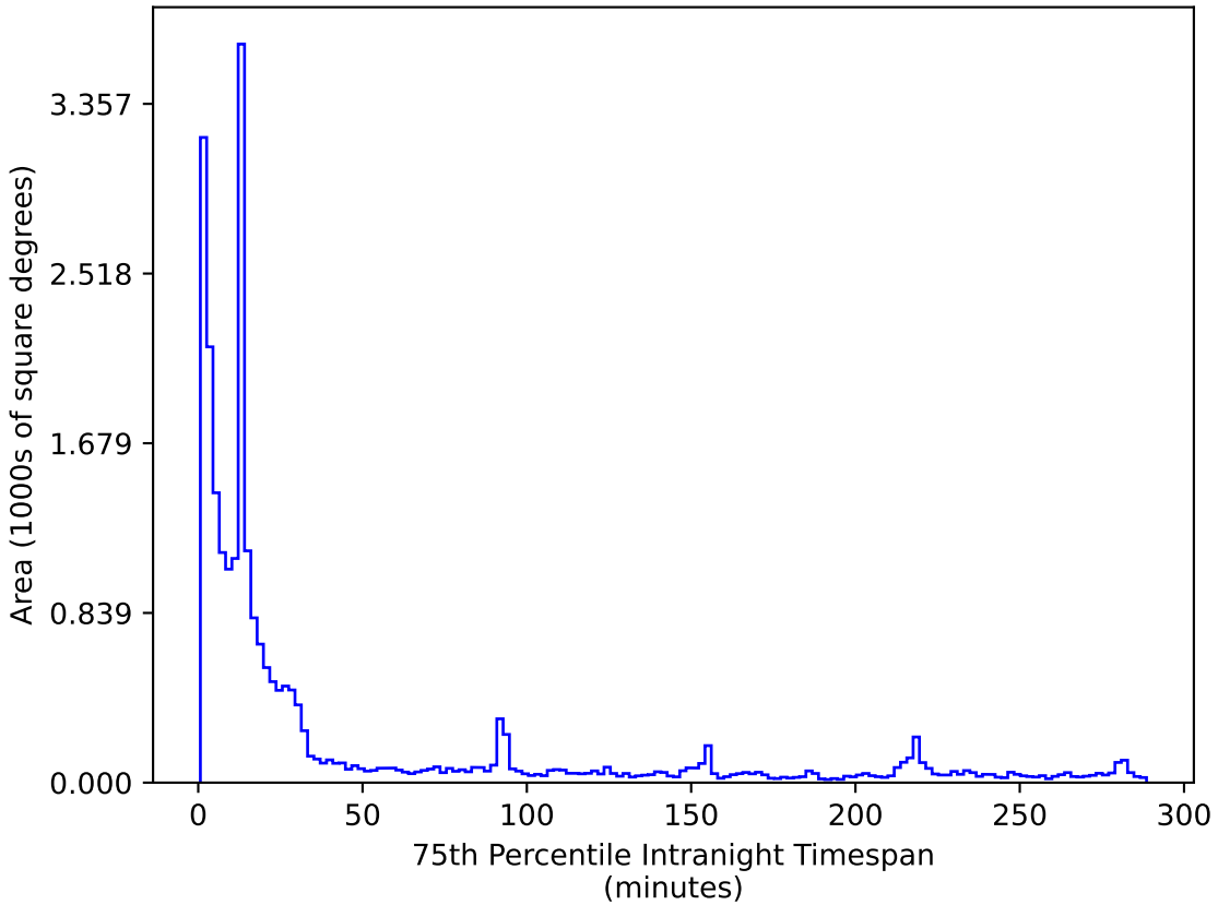
ddf_acor_sf15_lsf40_lsr20_v3.4_10yrs All sky r band: 75th Percentile Intranight Timespan
