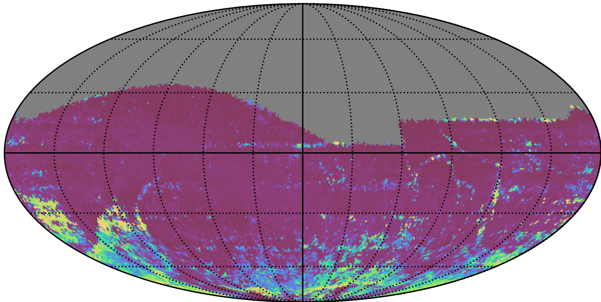
ddf_acor_sf15_lsf40_lsr20_v3.4_10yrs All sky i band: 75th Percentile Intranight Timespan
