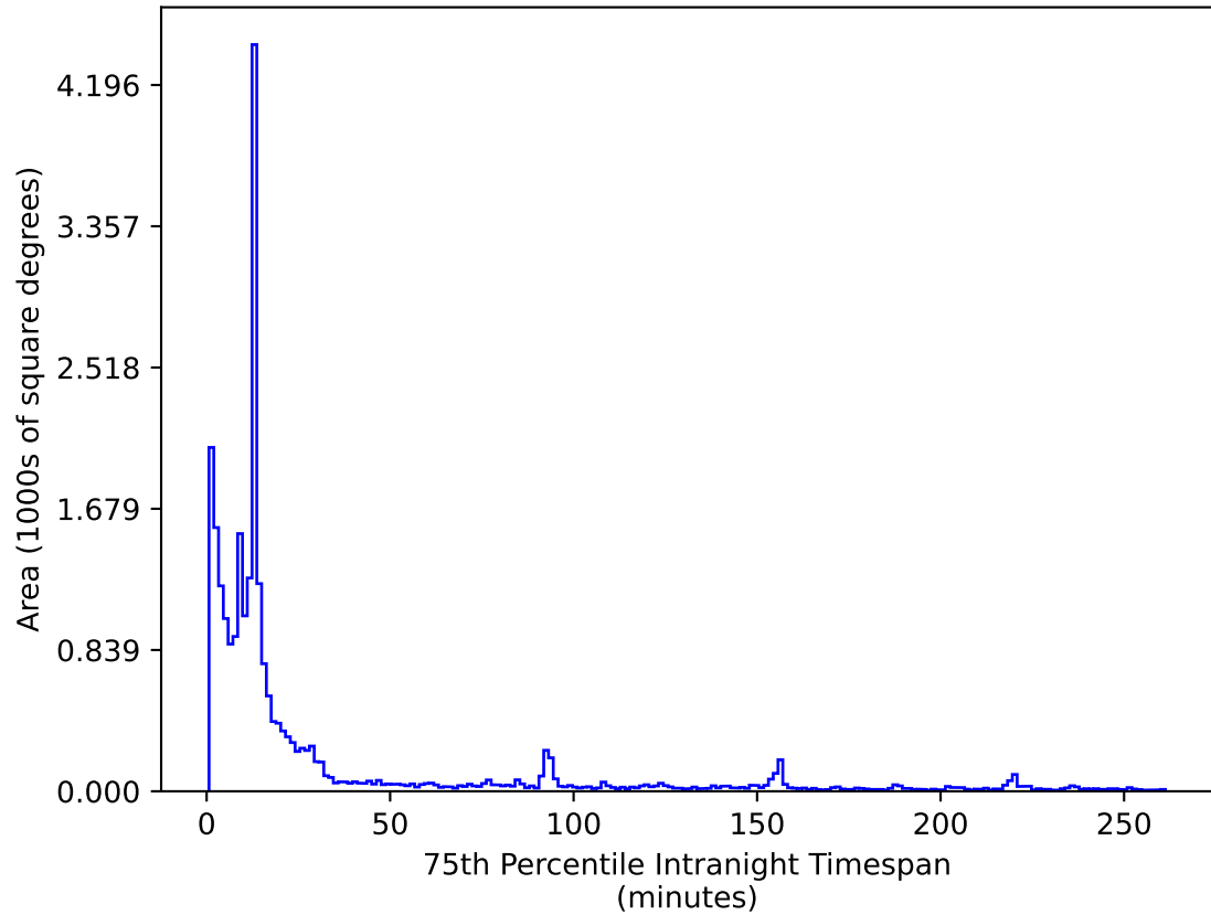
ddf_acor_sf15_lsf40_lsr20_v3.4_10yrs All sky i band: 75th Percentile Intranight Timespan
