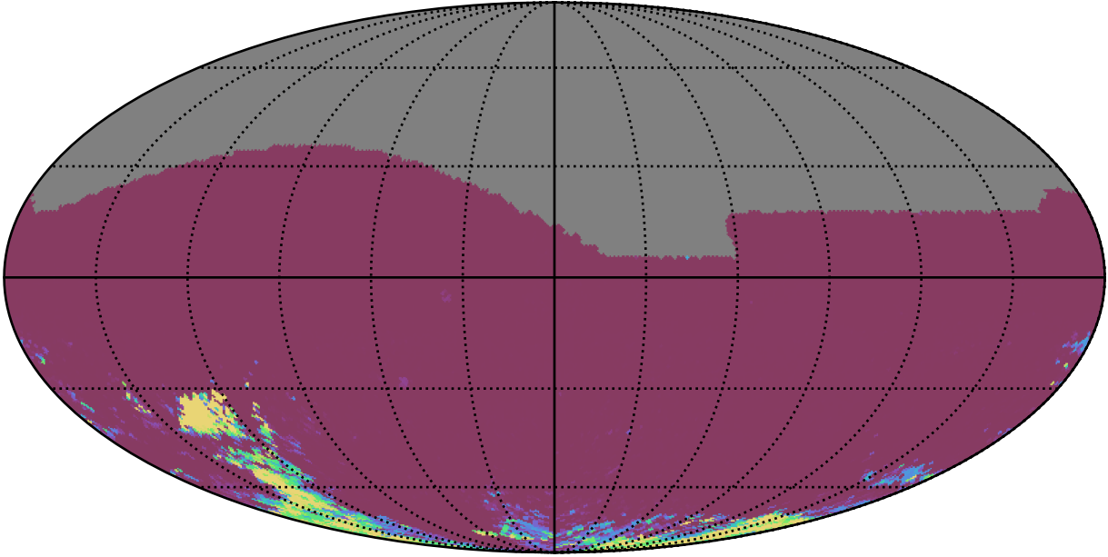
ddf_acor_sf15_lsf40_lsr20_v3.4_10yrs All sky gr bands: 75th Percentile Intranight Timespan
