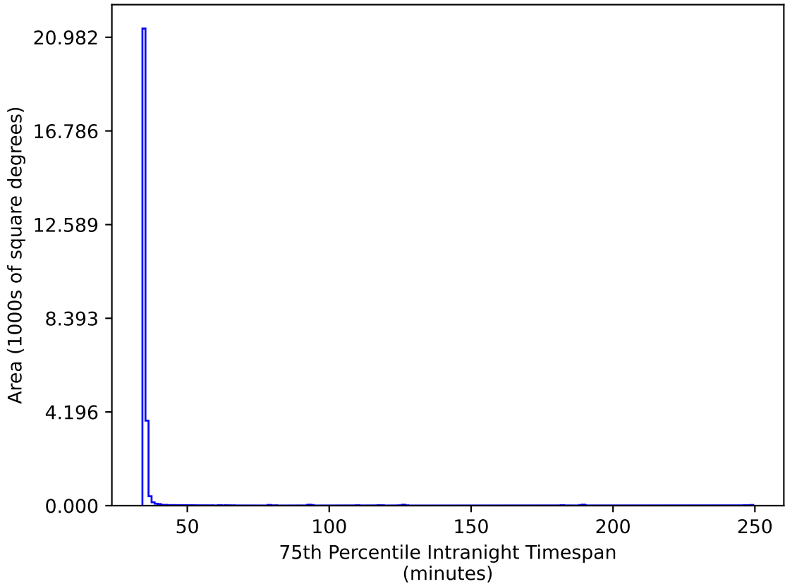
ddf_acor_sf15_lsf40_lsr20_v3.4_10yrs All sky gr bands: 75th Percentile Intranight Timespan
