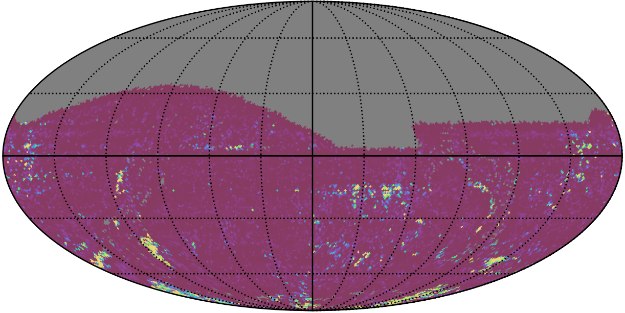
ddf_acor_sf15_lsf40_lsr20_v3.4_10yrs All sky g band: 75th Percentile Intranight Timespan
