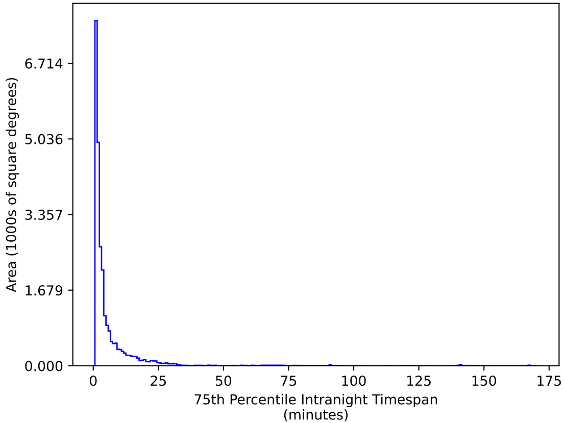
ddf_acor_sf15_lsf40_lsr20_v3.4_10yrs All sky g band: 75th Percentile Intranight Timespan
