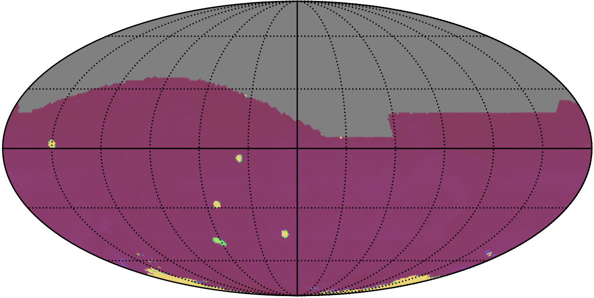
ddf_acor_sf15_lsf40_lsr20_v3.4_10yrs All sky all bands: 75th Percentile Intranight Timespan
