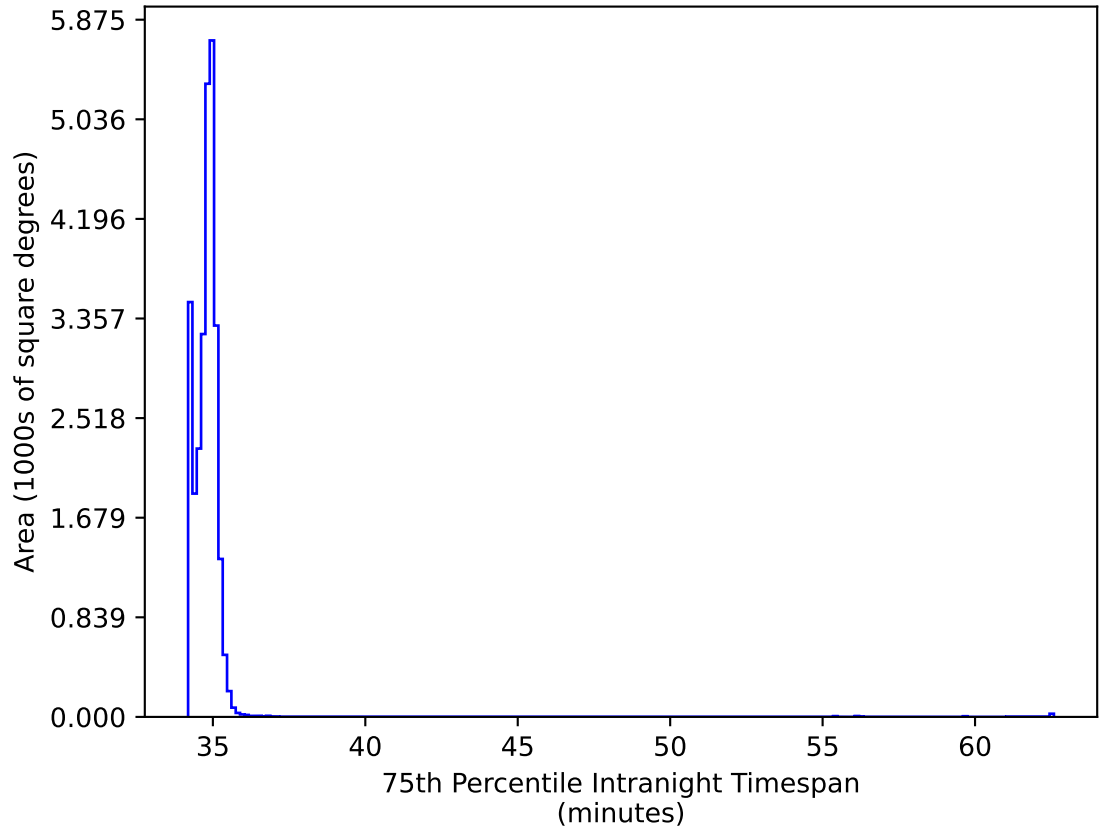
ddf_acor_sf15_lsf40_lsr20_v3.4_10yrs All sky: 75th Percentile Intranight Timespan
