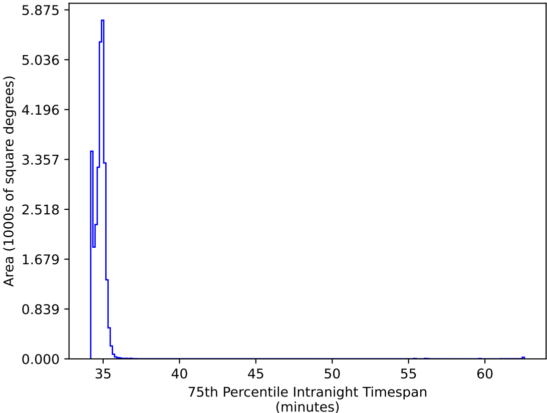
ddf_acor_sf15_lsf40_lsr20_v3.4_10yrs All sky: 75th Percentile Intranight Timespan
