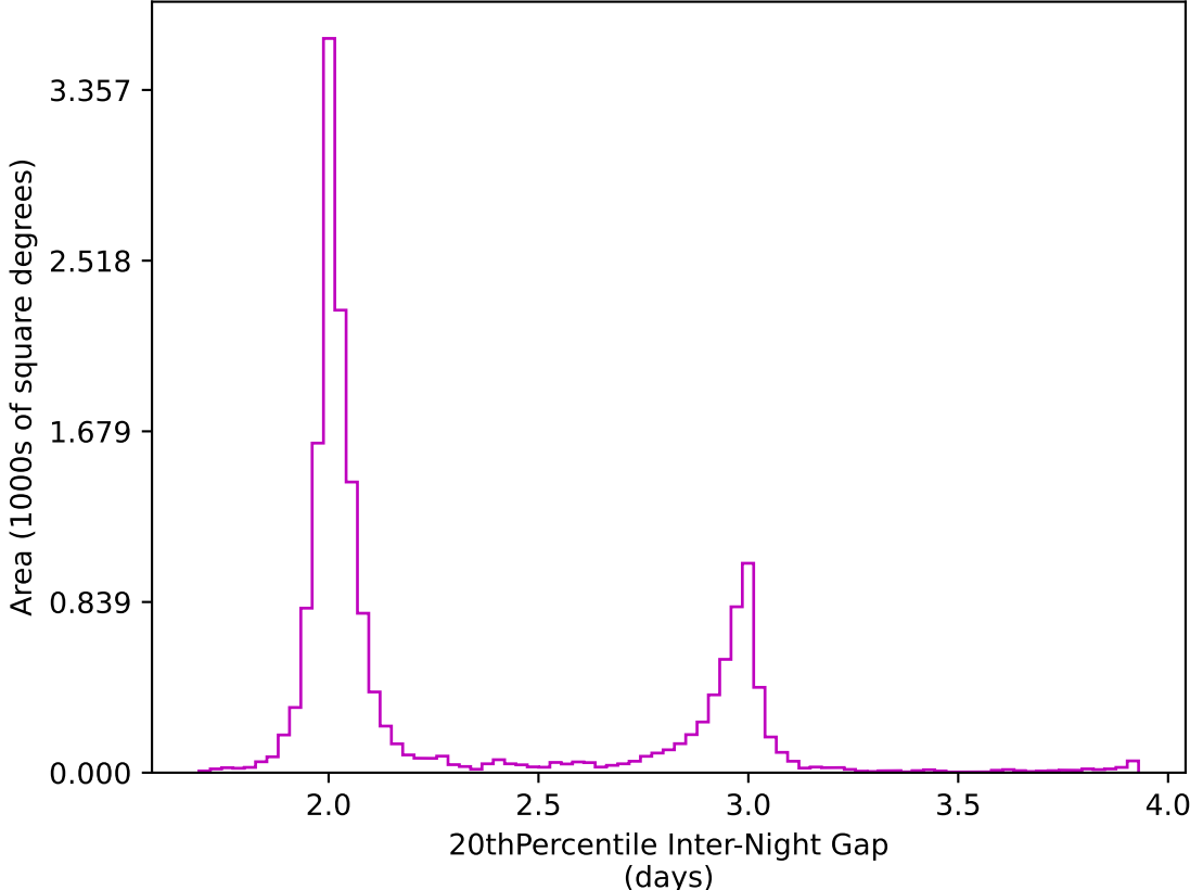
ddf_acor_sf15_lsf40_lsr20_v3.4_10yrs WFD z band: 20thPercentile Inter-Night Gap
