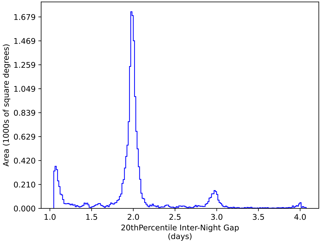
ddf_acor_sf15_lsf40_lsr20_v3.4_10yrs WFD y band: 20thPercentile Inter-Night Gap
