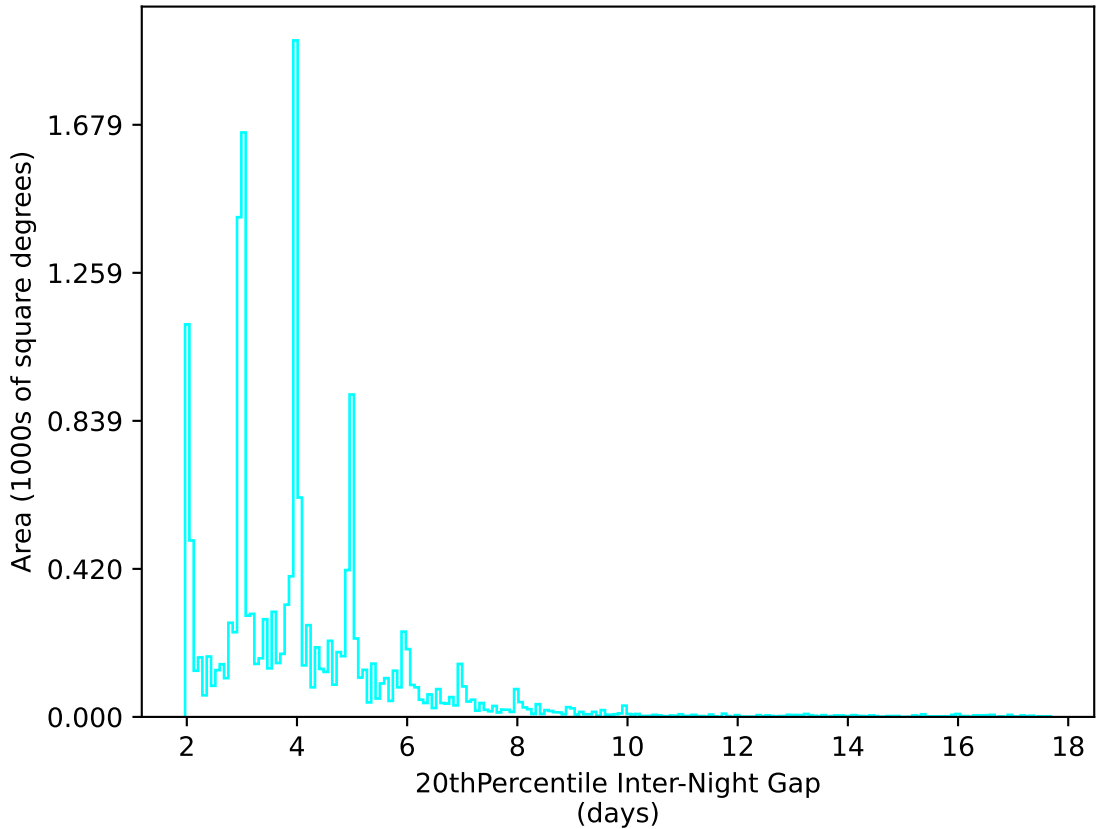
ddf_acor_sf15_lsf40_lsr20_v3.4_10yrs WFD u band: 20thPercentile Inter-Night Gap
