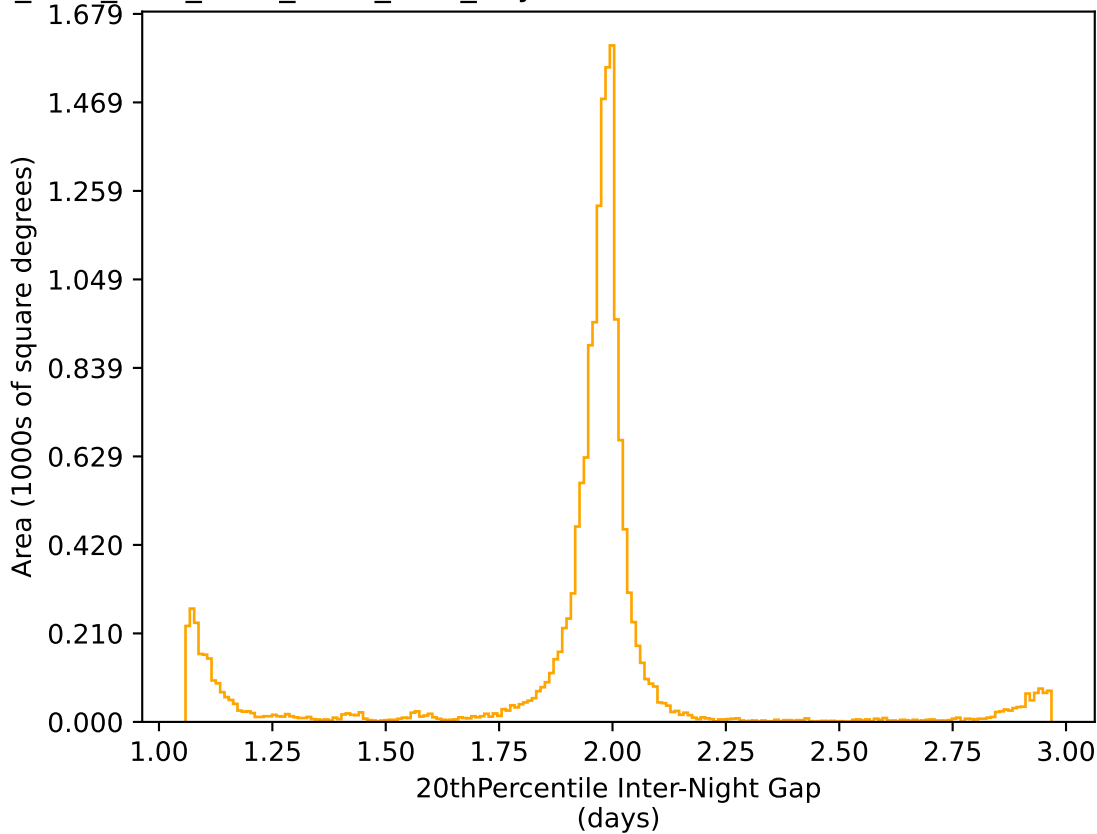
ddf_acor_sf15_lsf40_lsr20_v3.4_10yrs WFD r band: 20thPercentile Inter-Night Gap
