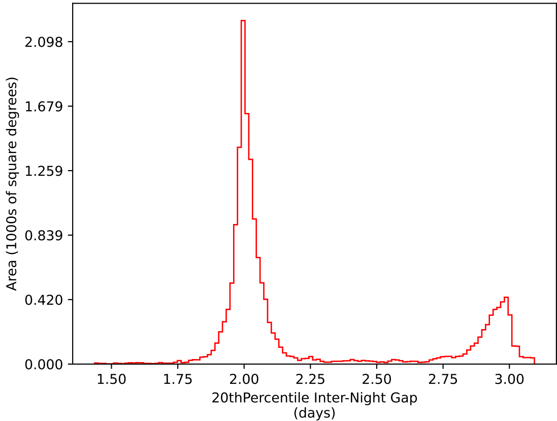
ddf_acor_sf15_lsf40_lsr20_v3.4_10yrs WFD i band: 20thPercentile Inter-Night Gap
