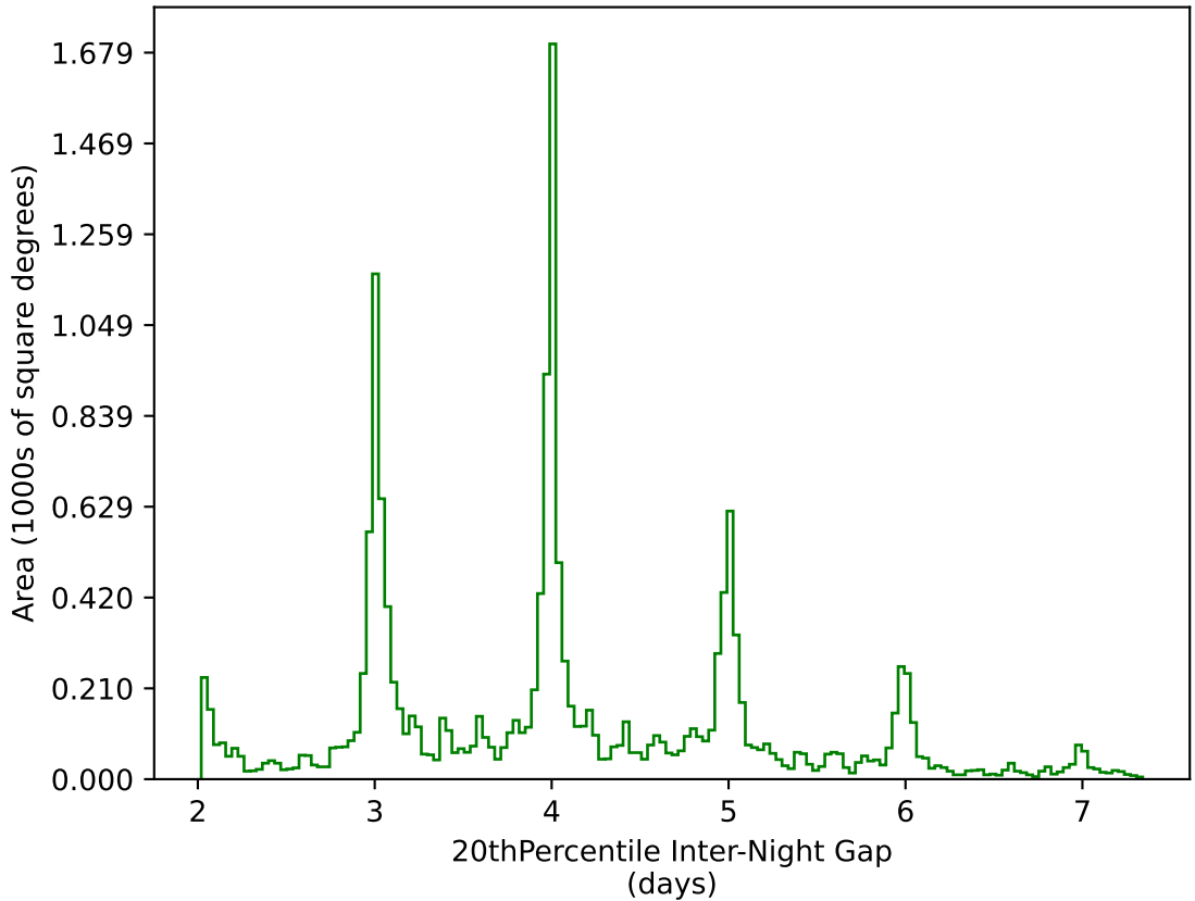
ddf_acor_sf15_lsf40_lsr20_v3.4_10yrs WFD g band: 20thPercentile Inter-Night Gap
