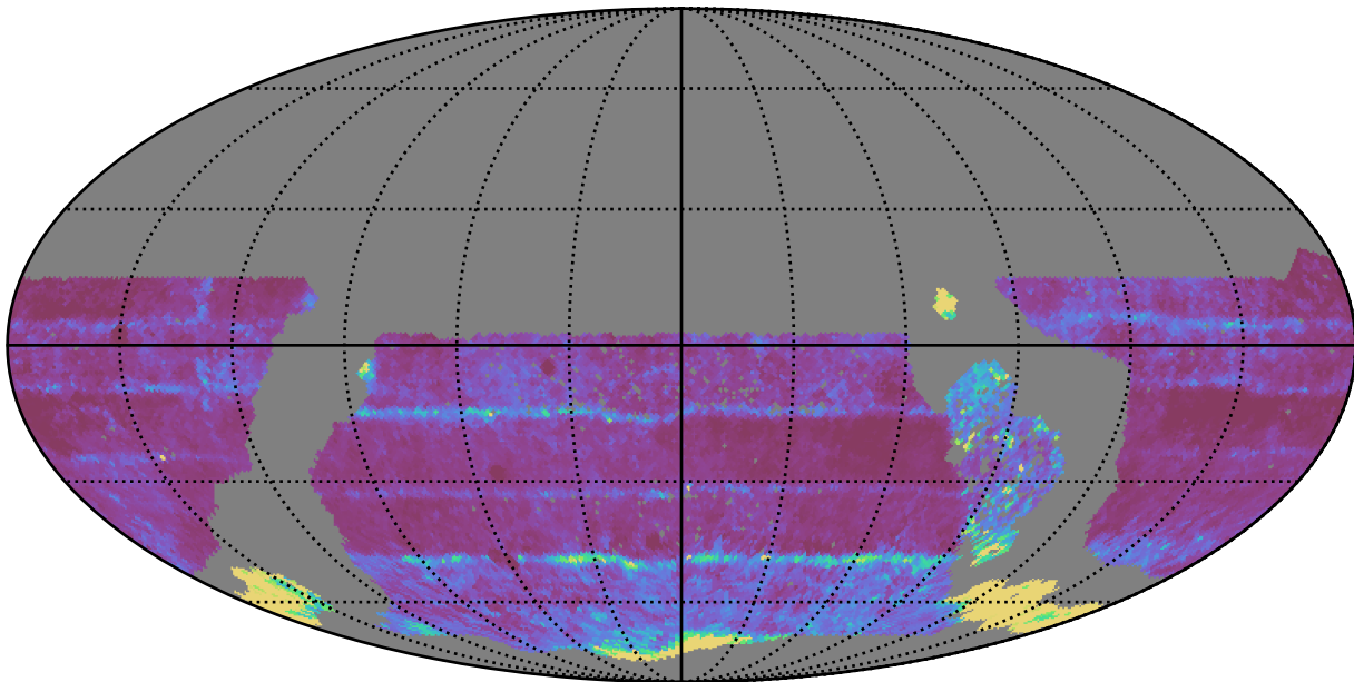
ddf_acor_sf15_lsf40_lsr20_v3.4_10yrs WFD all bands: 20thPercentile Inter-Night Gap
