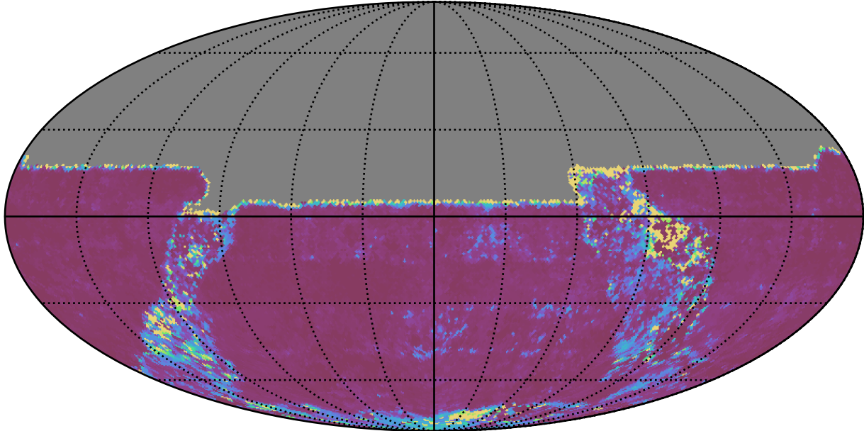
ddf_acor_sf15_lsf40_lsr20_v3.4_10yrs All sky u band: 20thPercentile Inter-Night Gap
