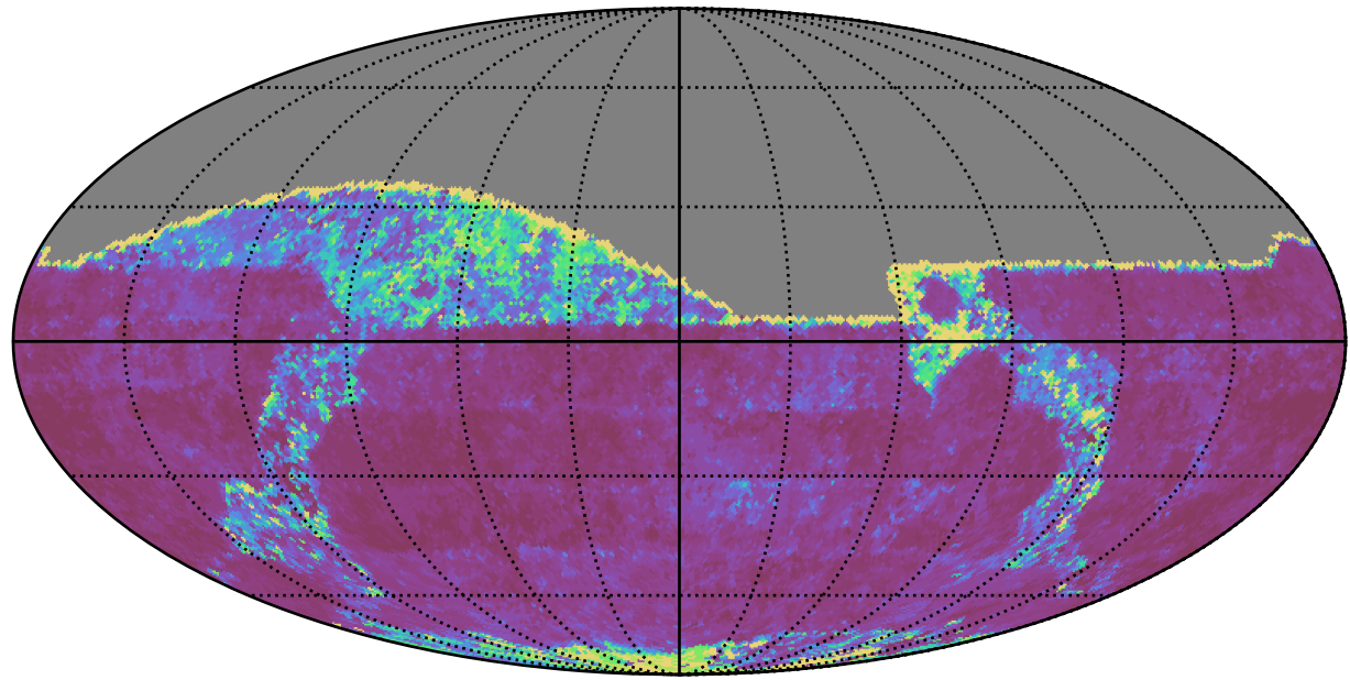
ddf_acor_sf15_lsf40_lsr20_v3.4_10yrs All sky g band: 20thPercentile Inter-Night Gap
