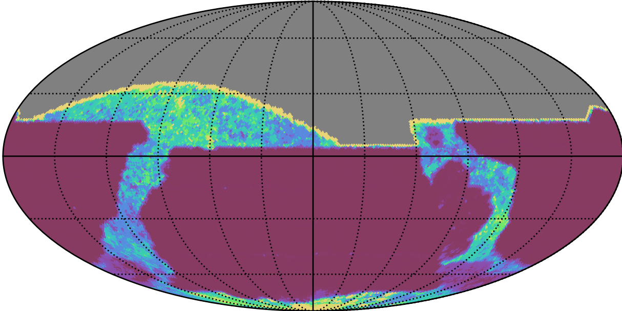
ddf_acor_sf15_lsf40_lsr20_v3.4_10yrs All sky all bands: 20thPercentile Inter-Night Gap
