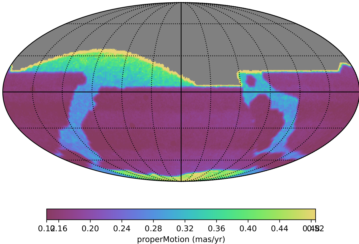
ddf_acor_sf15_lsf40_lsr20_v3.4_10yrs : properMotion
