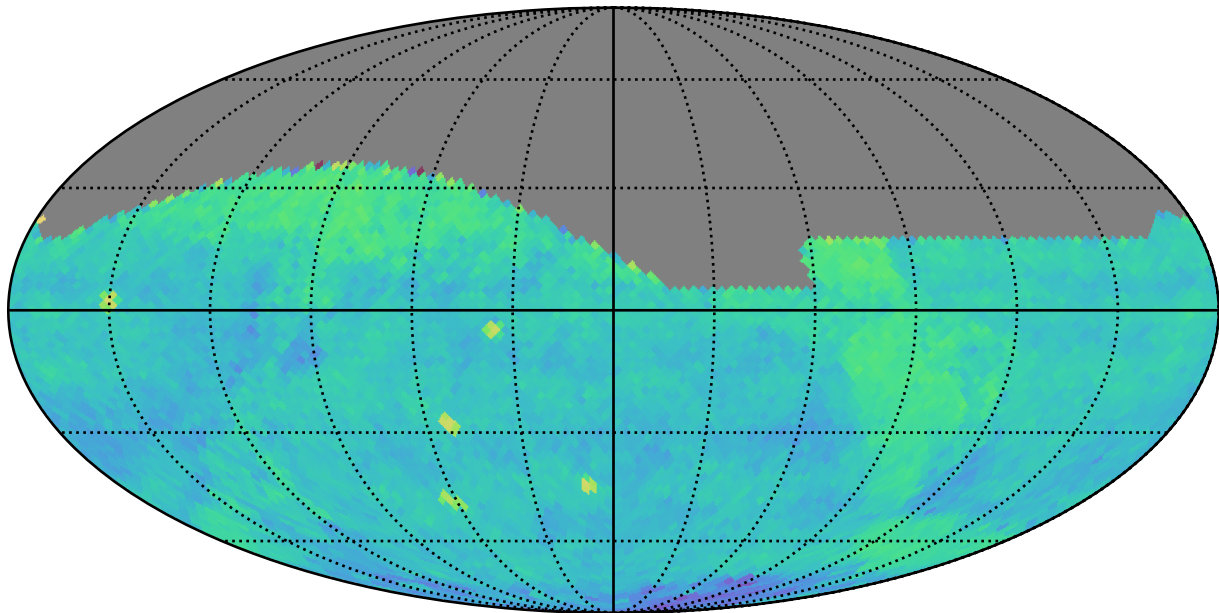
ddf_acor_sf15_lsf40_lsr20_v3.4_10yrs (g or r or i): PairFraction
