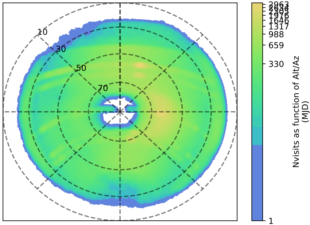
ddf_acor_sf15_lsf40_lsr20_v3.4_10yrs z: Nvisits as function of Alt/Az
