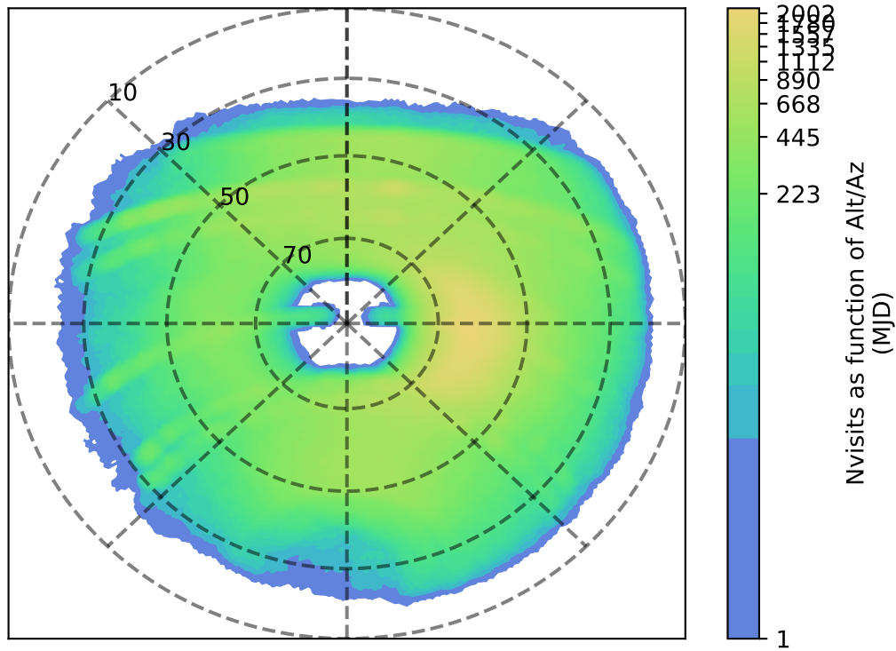
ddf_acor_sf15_lsf40_lsr20_v3.4_10yrs y: Nvisits as function of Alt/Az
