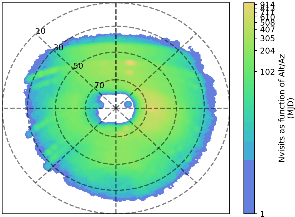
ddf_acor_sf15_lsf40_lsr20_v3.4_10yrs u: Nvisits as function of Alt/Az
