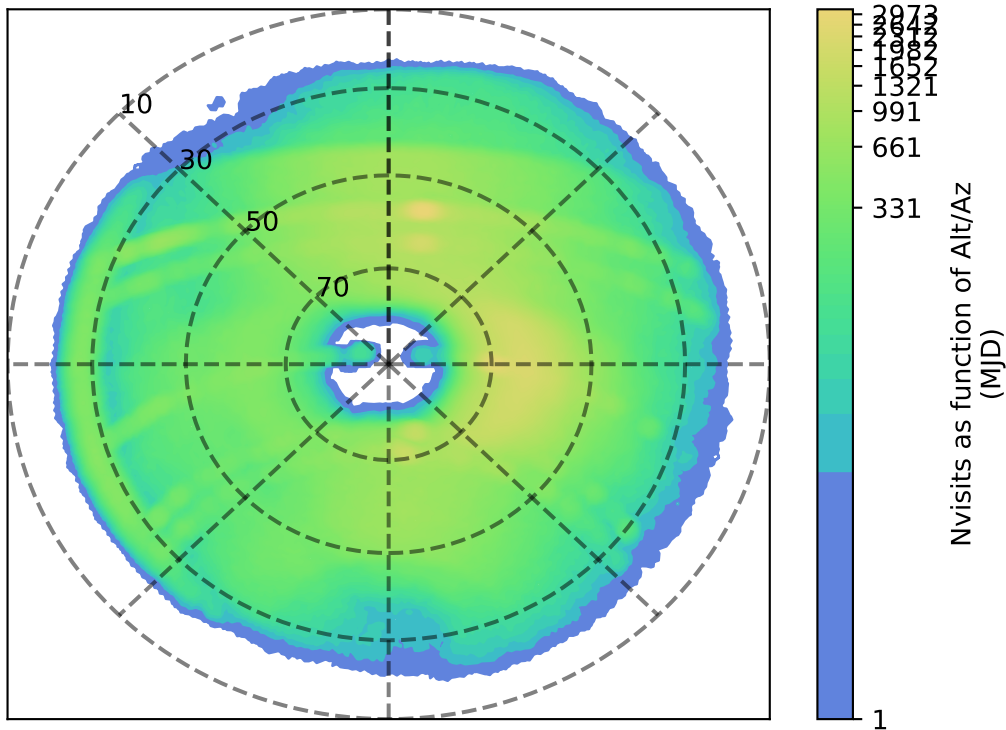
ddf_acor_sf15_lsf40_lsr20_v3.4_10yrs r: Nvisits as function of Alt/Az
