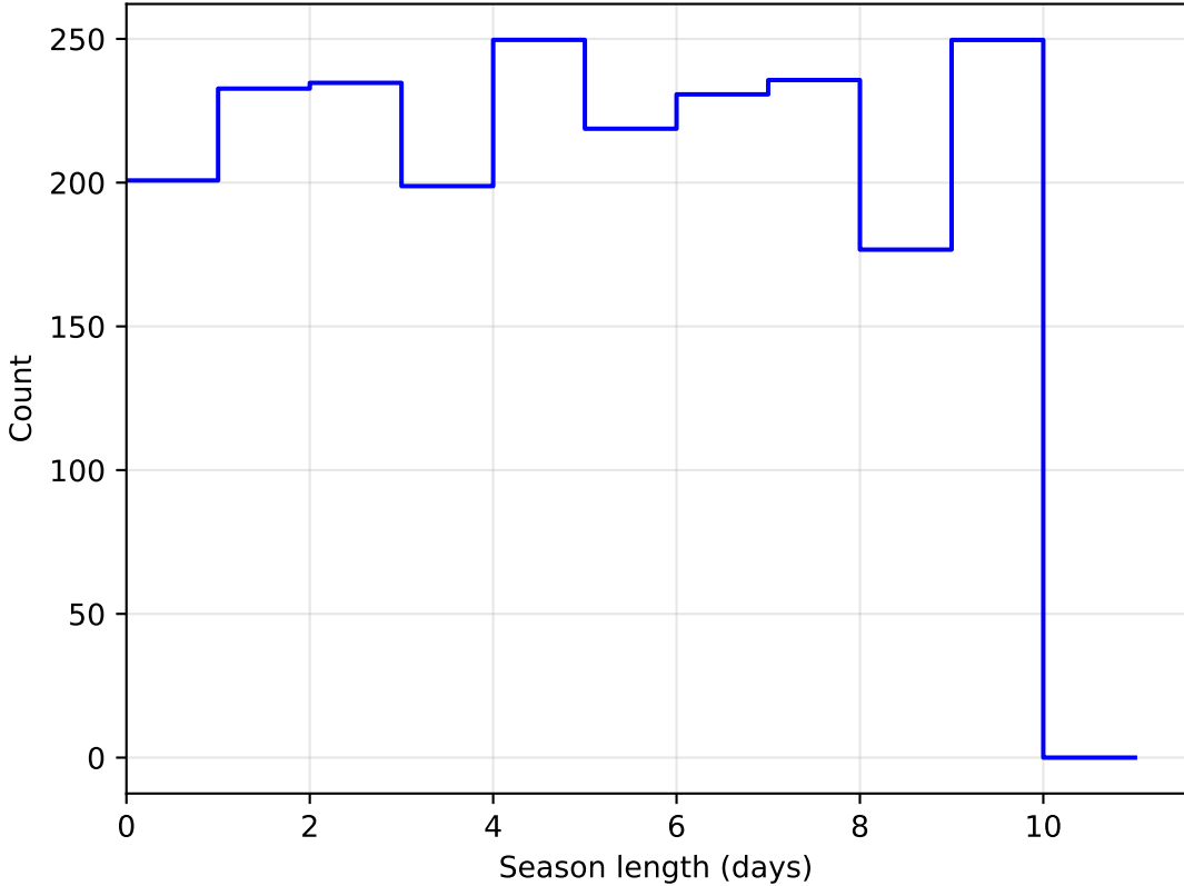
ddf_acor_sf15_lsf40_lsr20_v3.4_10yrs DD:XMM_LSS all bands: SeasonLength
