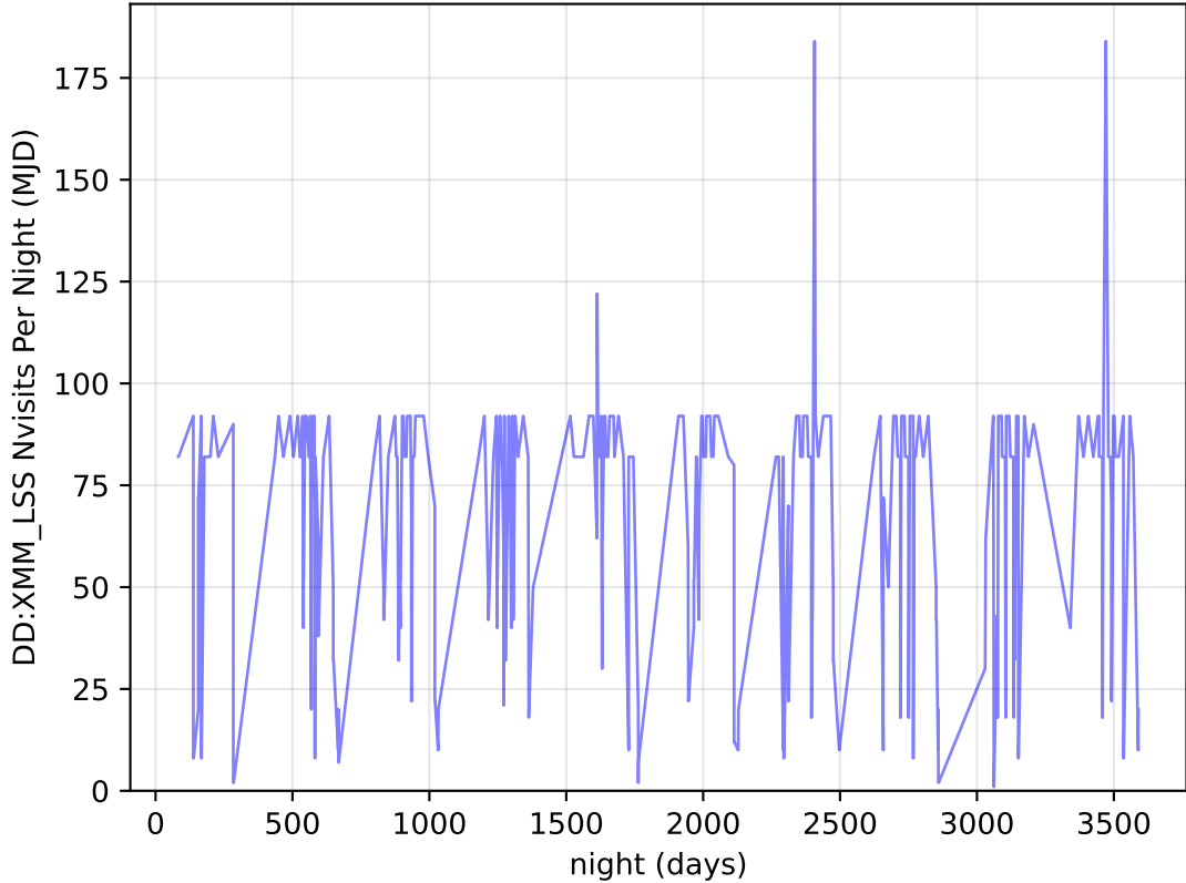
ddf_acor_sf15_lsf40_lsr20_v3.4_10yrs all bands: DD:XMM_LSS Nvisits Per Night
