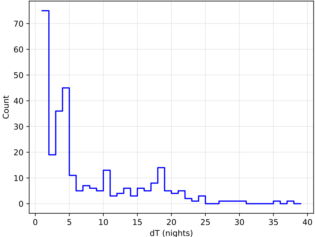
ddf_acor_sf15_Isf40_Isr20_v3.4_10yrs all bands: DD:XMM_LSS Delta Nights Histogram
