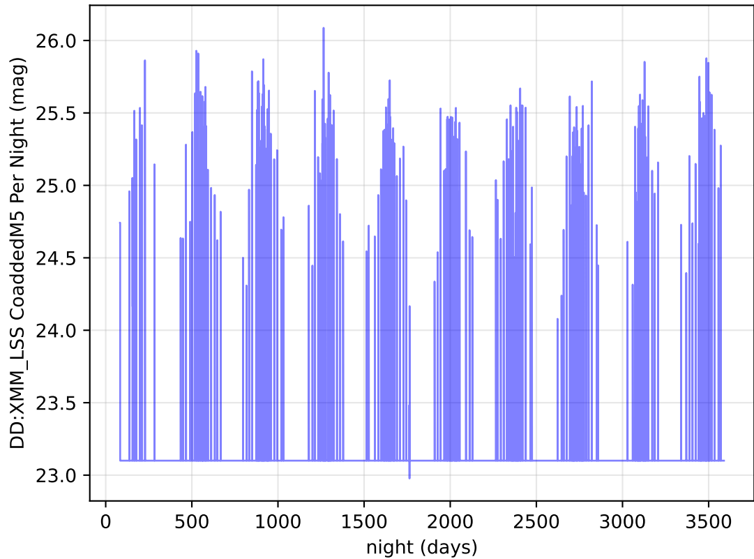
ddf_acor_sf15_lsf40_lsr20_v3.4_10yrs i band: DD:XMM_LSS CoaddedM5 Per Night
