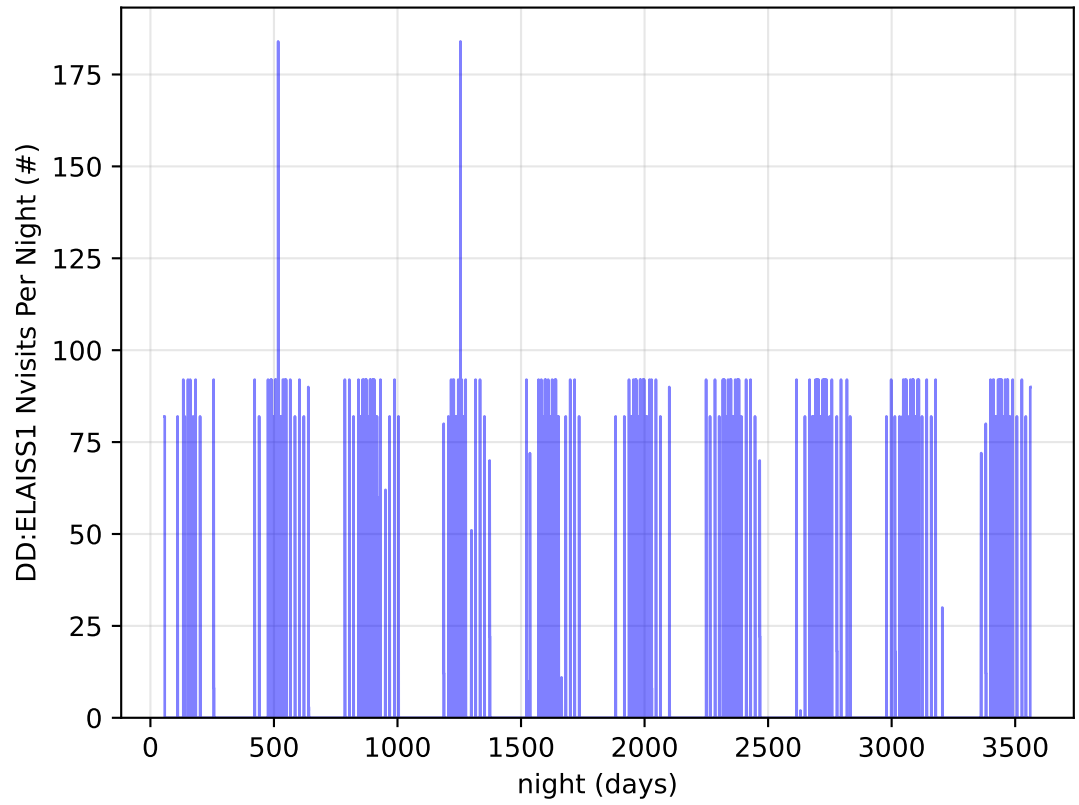
ddf_acor_sf15_ls40_lsr20_v3.4_10yrs all bands: DD:ELAISS1 Nvisits Per Night
