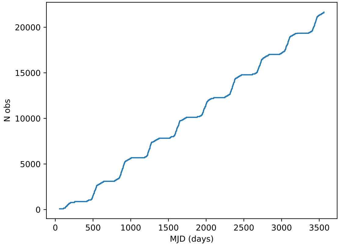
ddf_acor_sf15_lsf40_lsr20_v3.4_10yrs all bands: DD:ELAISS1 Cumulative NVisits
