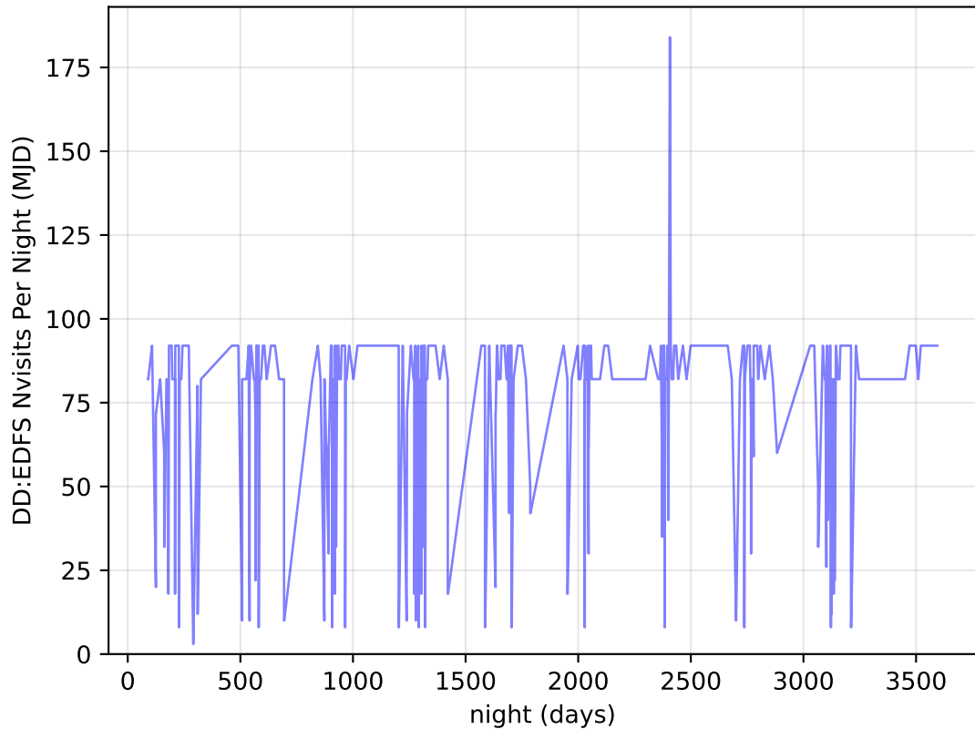
ddf_acor_sf15_lsf40_lsr20_v3.4_10yrs all bands: DD:EDFS Nvisits Per Night
