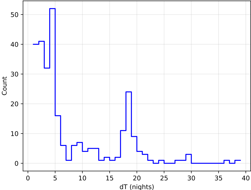
ddf_acor_sf15_lsf40_lsr20_v3.4_10yrs all bands: DD:EDFS Delta Nights Histogram
