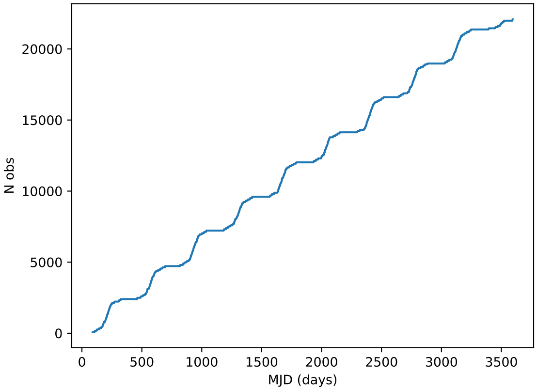
ddf_acor_sf15_lsf40_lsr20_v3.4_10yrs all bands: DD:EDFS Cumulative NVisits
