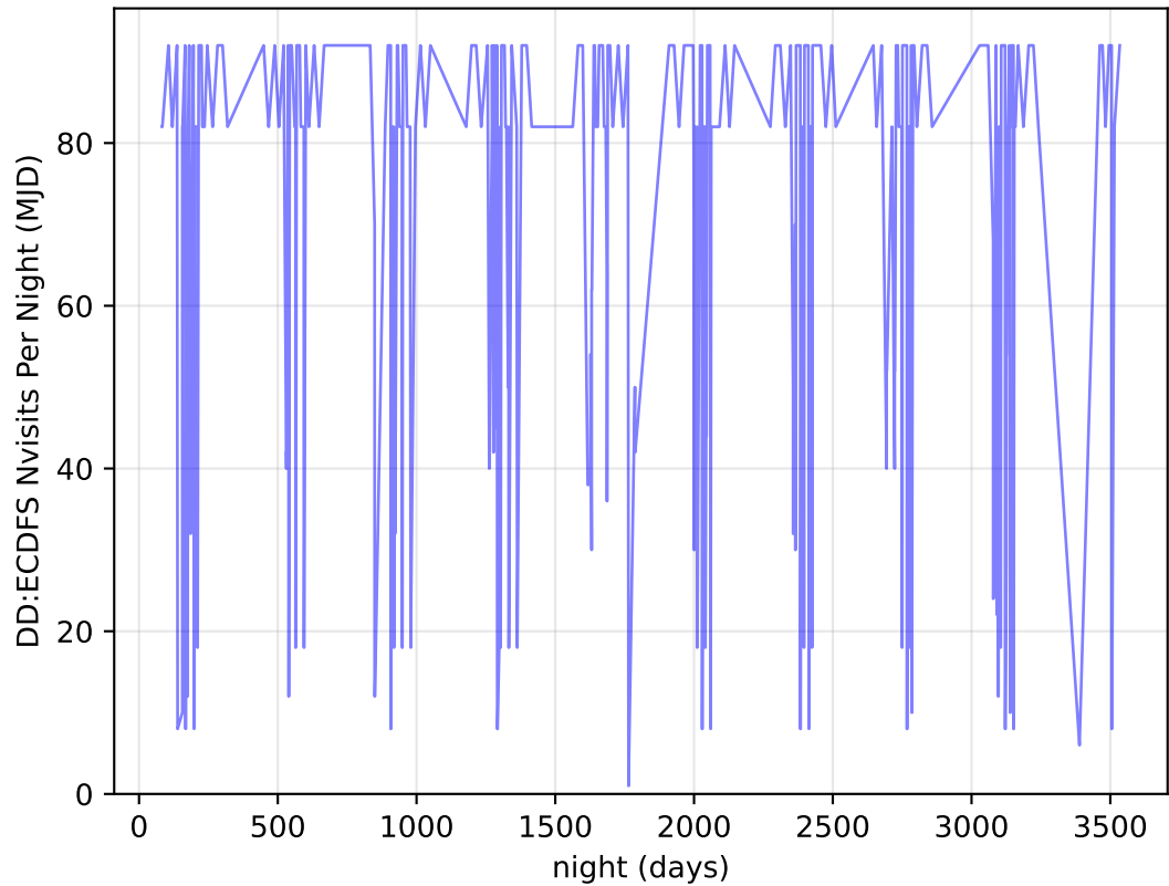
ddf_acor_sf15_lsf40_lsr20_v3.4_10yrs all bands: DD:ECDFS Nvisits Per Night
