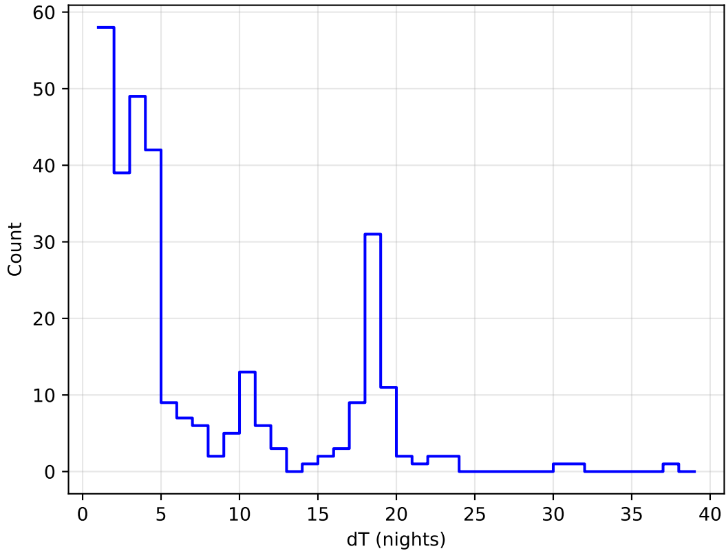
ddf_acor_sf15_lsf40_lsr20_v3.4_10yrs all bands: DD:ECDFS Delta Nights Histogram
