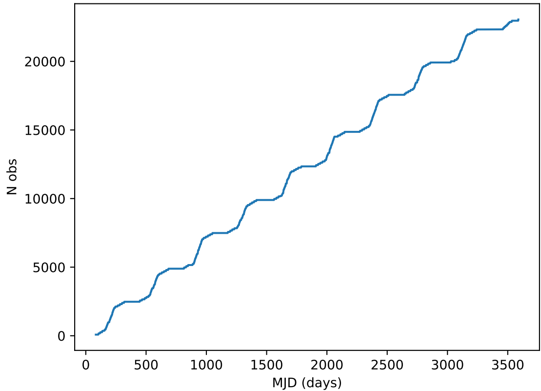
ddf_acor_sf15_lsf40_lsr20_v3.4_10yrs all bands: DD:ECDFS Cumulative NVisits
