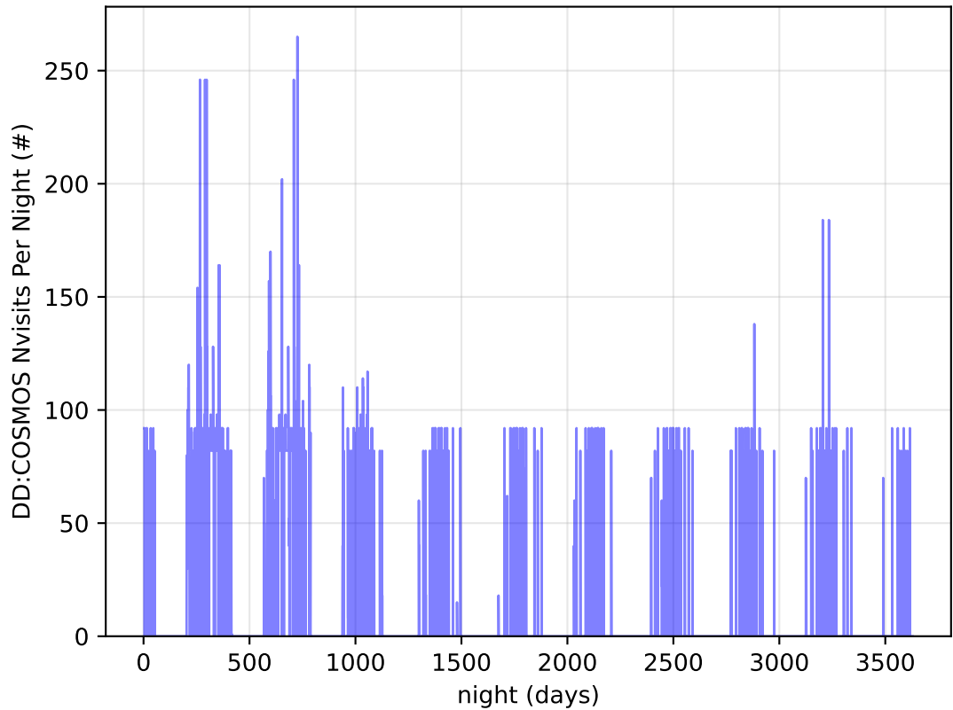
ddf_acor_sf15_lsf40_lsr20_v3.4_10yrs all bands: DD:COSMOS Nvisits Per Night
