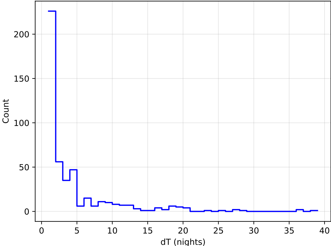
ddf_acor_sf15_Isf40_Isr20_v3.4_10yrs all bands: DD: COSMOS Delta Nights Histogram
