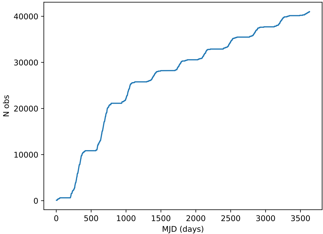
ddf_acor_sf15_lsf40_lsr20_v3.4_10yrs all bands: DD: COSMOS Cumulative NVisits
